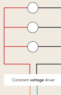
constant voltage parallel wiring
