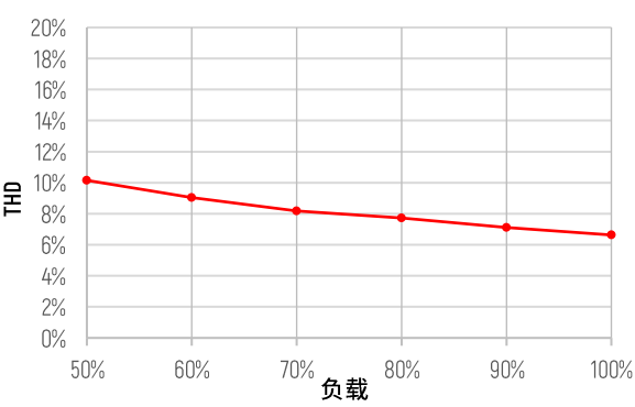
THD vs. 负载
