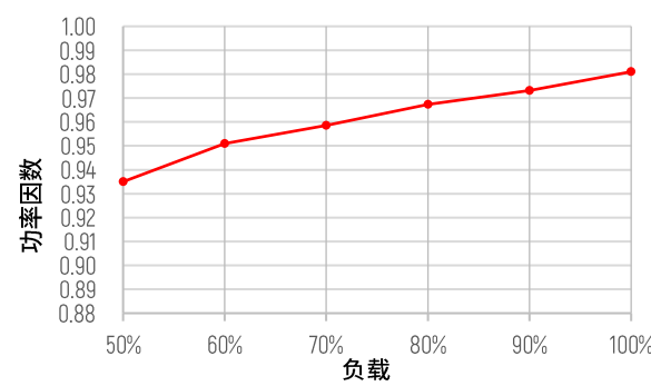
PF vs. 负载
