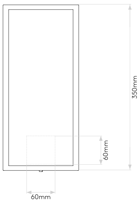
Recess in wall for Terminal Block 60x60x30mm
